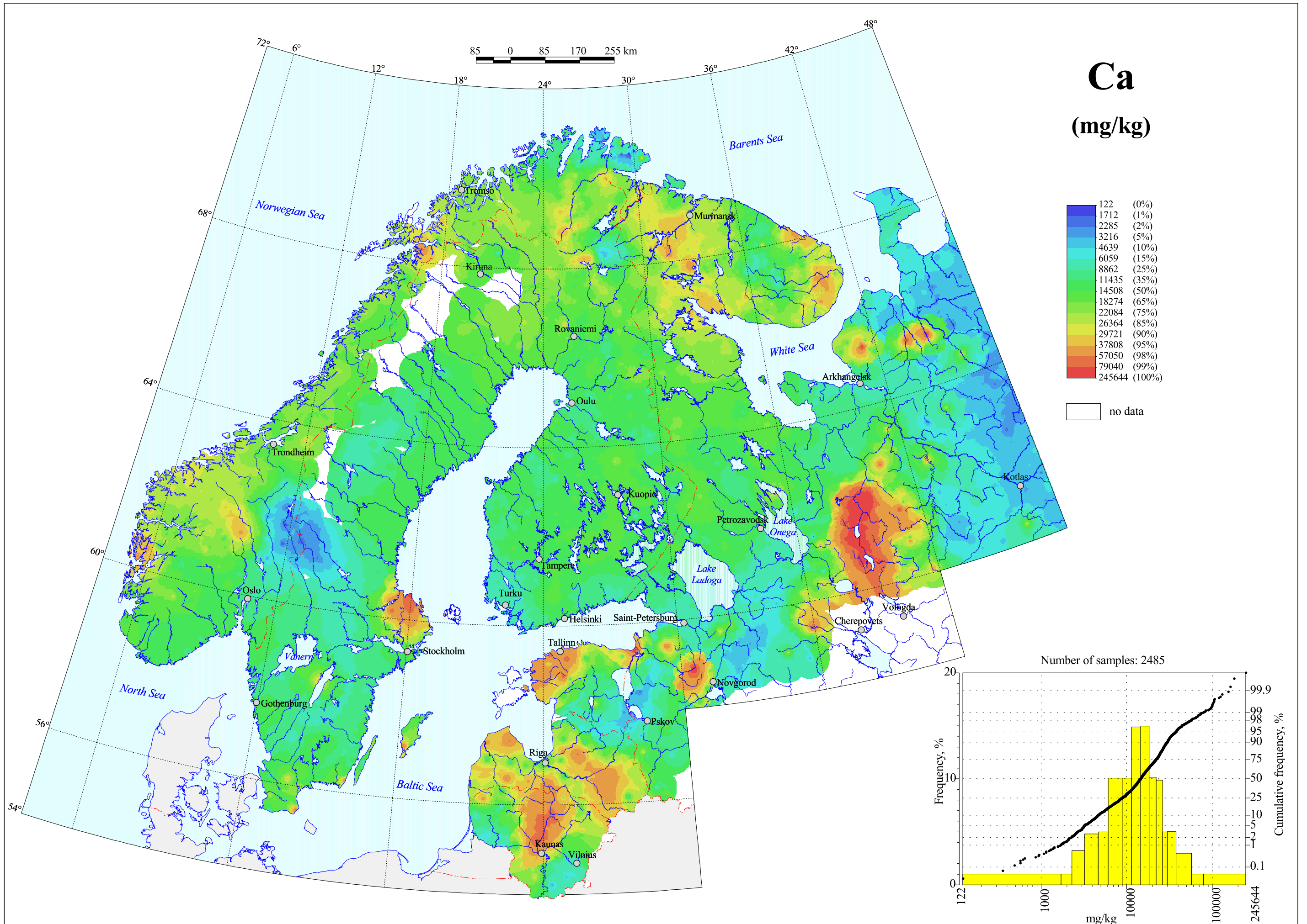
Calcium in C-horizon, Grain Size <2 mm, Total Content
